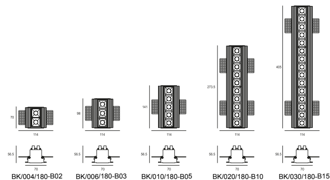
BK/004/180-B02 BK/006/180-B03 BK/010/180-B05 BK/020/180-B10 BK/030/180-B15
